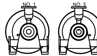
ASSEMBLY DIAGRAMS FACING DRIVE END ASSEMBLY NO. 1 IS STANDARD WITH CLOCKWISE ROTATION
