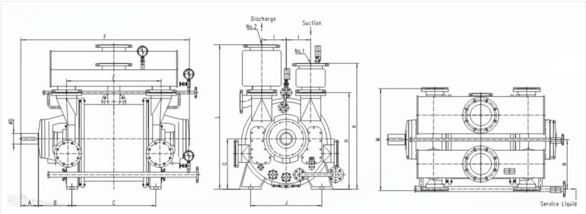
DIMENSIONS, KEYWAY & SHAFT DATA — DIMENSIONS IN MM
